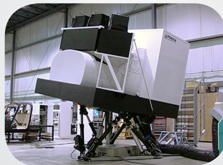
Level B Caravan FFS in use at the University of Alaska. Features 6-axis motion base. First Electric Motion Full Flight Simulator - 2003
